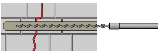
Spirallanker eindrehen | Screw-in spiral anchor
