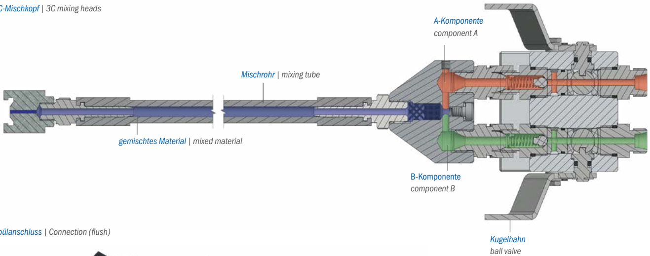
3C-Mischkopf | 3C mixing heads
